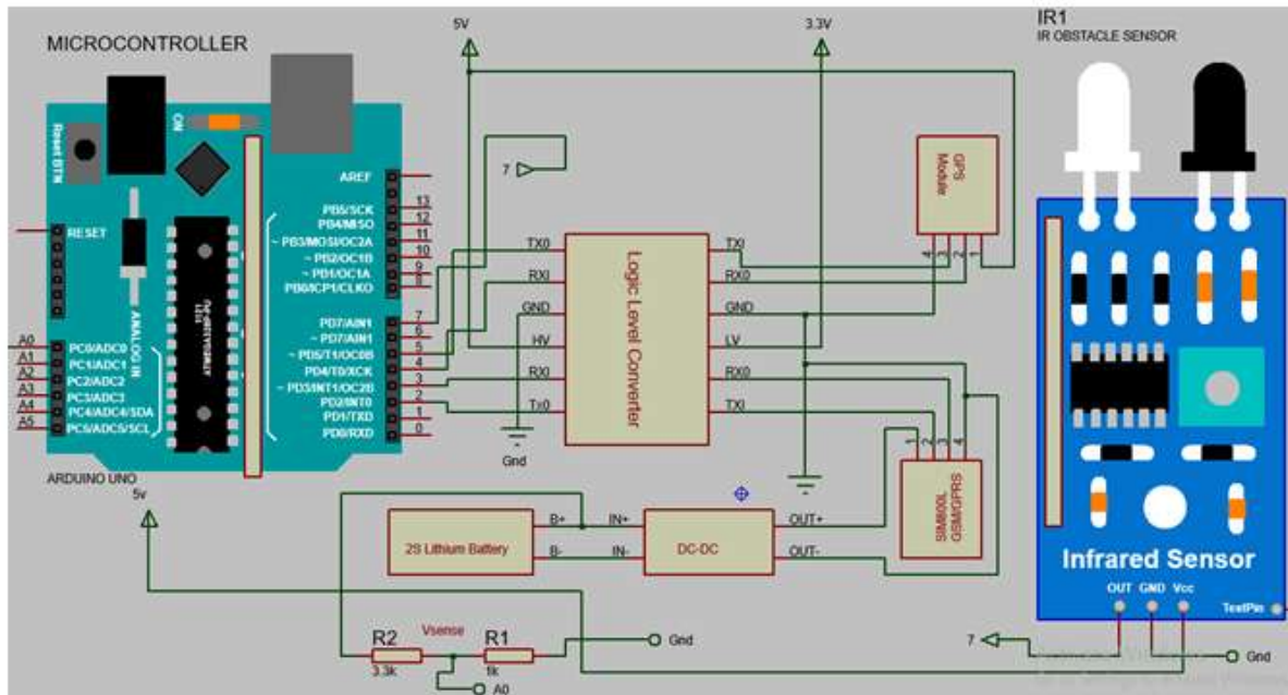
Fig. 1: Circuit Diagram
