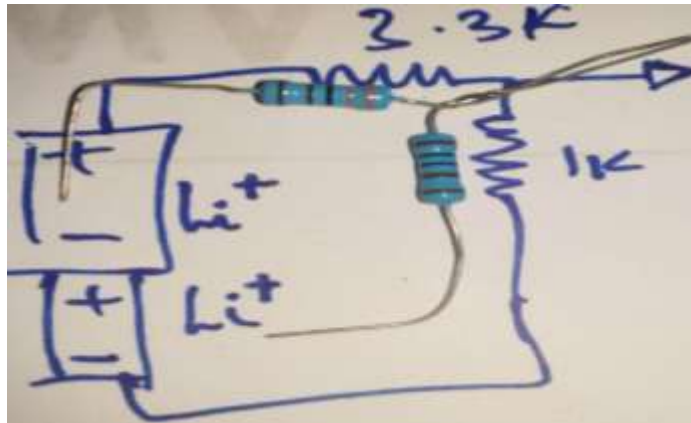
Fig. 3: Voltage measurement circuit
