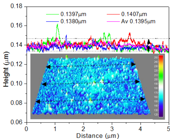
Figure 2. Line profiles showing topographical heights on \text{TiO}_2 film annealed at 1^{\circ}\text{C}/\text{min} (Inset- 3D image with lines where profiles were obtained)
