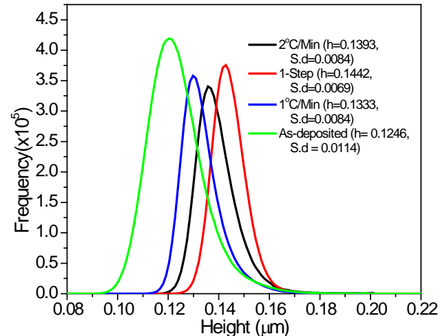
Figure 3. Histogram distributions on \text{TiO}_2 films annealed at different rates
