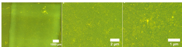
Figure 1. \text{TiO}_2 film on FTO glass annealed at 1^{\circ}\text{C}/\text{min} obtained at (a) 16, (b) 100 and (c) 260X magnifications
