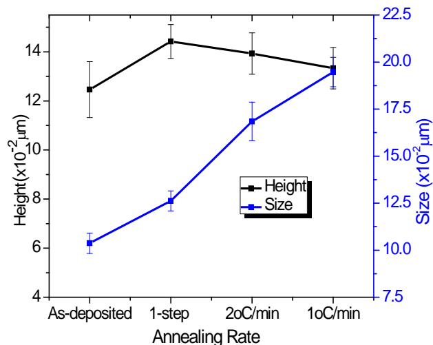
Figure 4. Variation of mean heights and sizes of the islands with annealing rate
