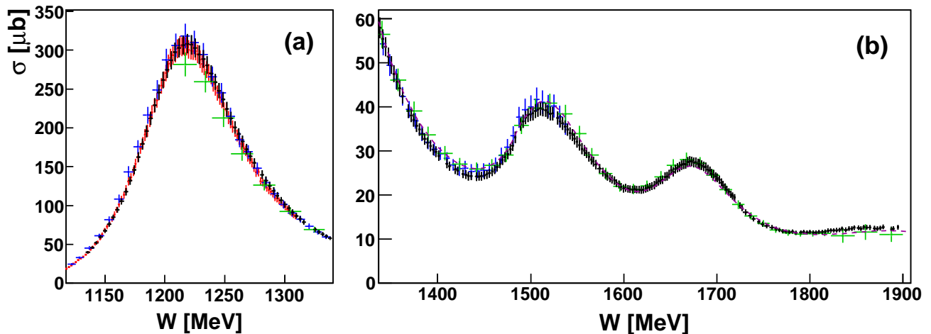
FIG. 6: (Color online) Total cross sections for \gamma p \rightarrow \pi^0 p from this work (black points) as a function of the c.m. energy W compared with earlier A2 results [25] (red points), with results from Refs. [26] (blue points) and [28] (green points), and with the SAID solution CM12 [24] shown in (b) by a magenta dashed line. For a better comparison, the energy range is divided in two intervals: (a) W < 1340 MeV and (b) W > 1340 MeV. The error bars on the experimental data points represent their total uncertainties.
