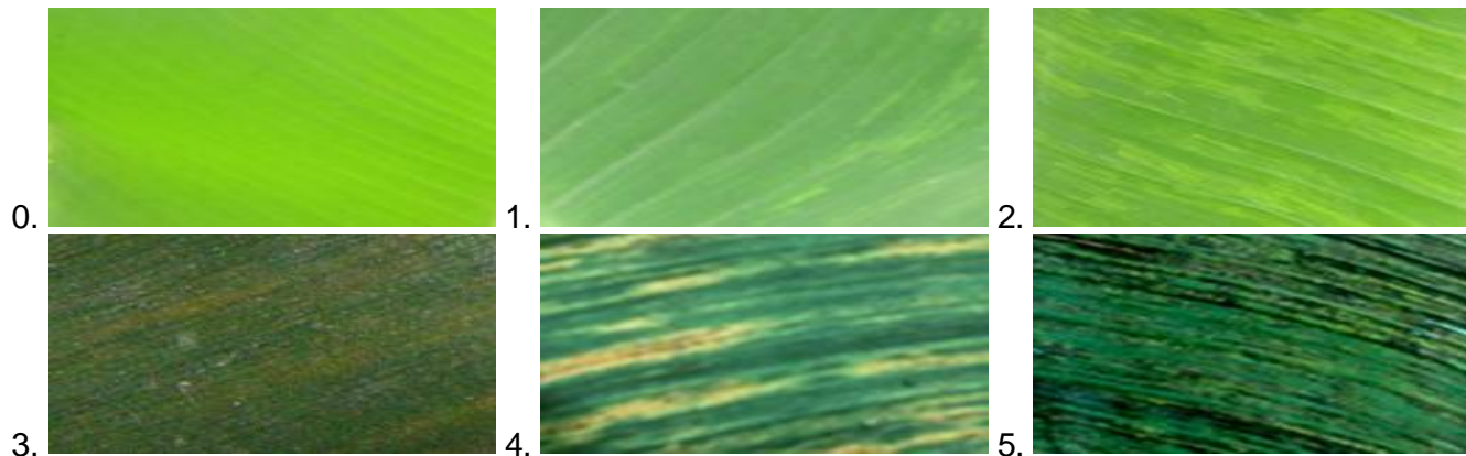
Figure 1. Banana leaves depicting symptoms severity scoring scale. 0 is no symptoms, 1 is localised flecks, 2 is scattered discontinuous streaks, 3 is continuous streaks covering moderate portion of lamina, 4 is continuous and conspicuous chlorotic streaks, 5 is necrotic streaks according to Karanja (2009).
