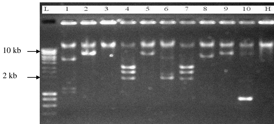
Figure 2. TempliPhi-RFLP for samples 1 to 10 using Stu1 . Lane H represents a healthy (negative) control (DNA extract of a BSD-free Musa tissue). Lane L is a molecular marker (Bioline Hyperladder).
