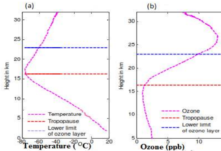
Fig. 3. Mean Vertical variation; (a) temperature, (b) Ozone over Nairobi 2011 to 2014
