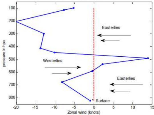
Fig. 5. Profile of zonal wind component for Nairobi, 2011 to 2014
