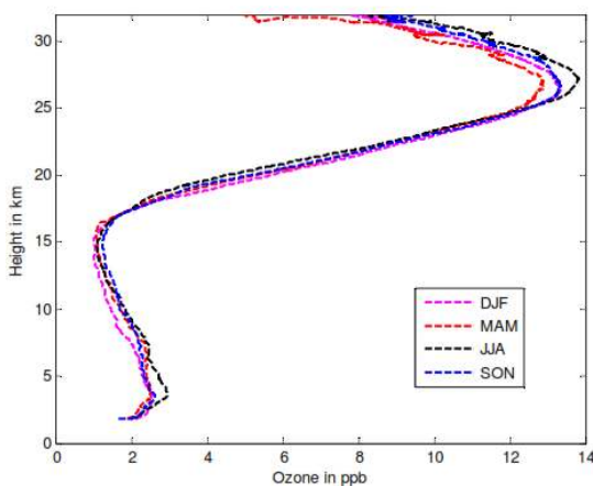
Fig. 4. Mean Vertical seasonal variation of Ozone over Nairobi, 2011 to 2014
