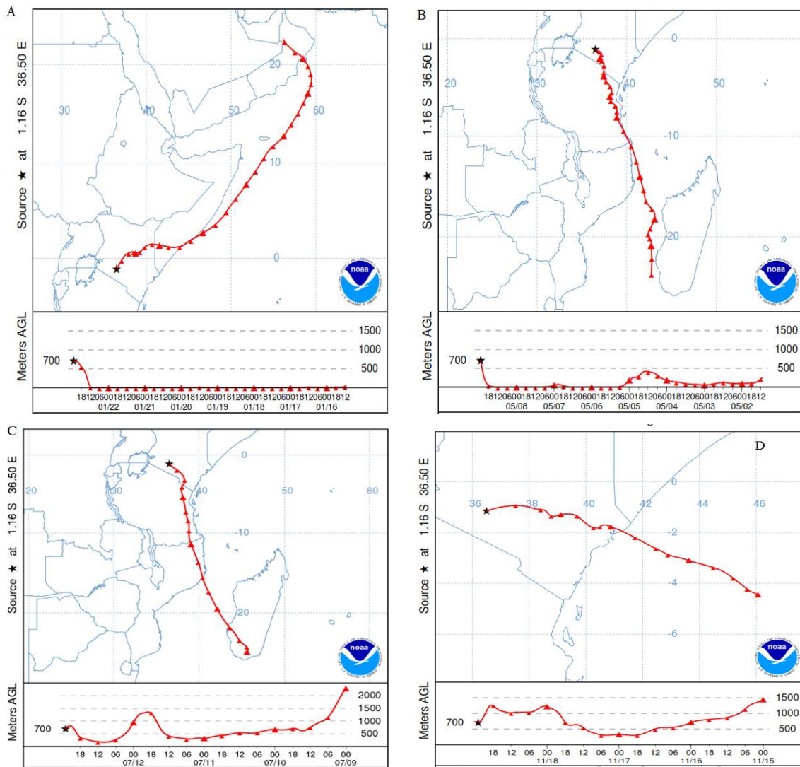
Fig. 7. Mean backward trajectories ending at Nairobi. The ending point height is 700 m, for (A) January (B) May (C) July (D) November
